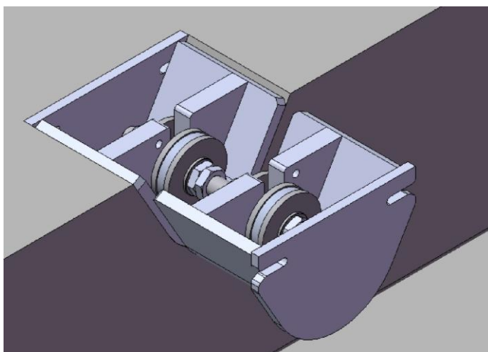
Figure A2.8: Horizontal connection placed on top horizontal surface of the units (solution 1).
