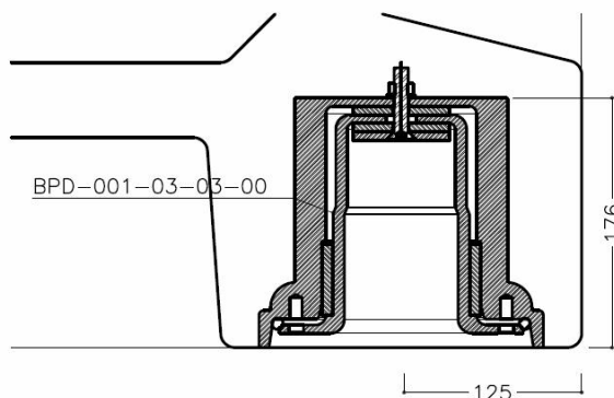
Figure A3.1: Cross-section of longitudinal floor beam of the unit.
