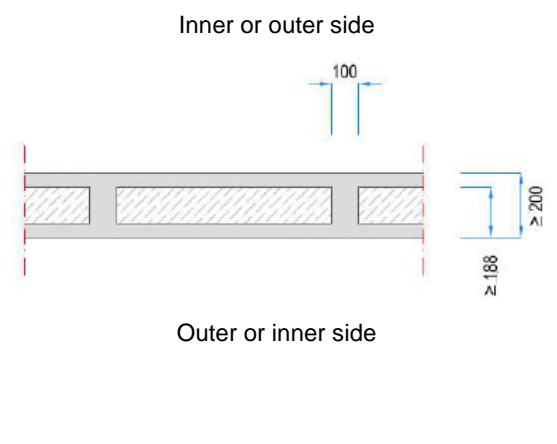
Figure 2. Structural sections of the Compact Habit ® unit.
